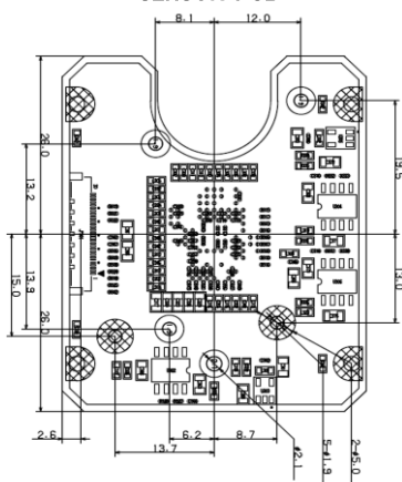
SENSOR-PCB
