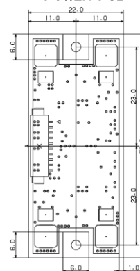
POWER-PCB
