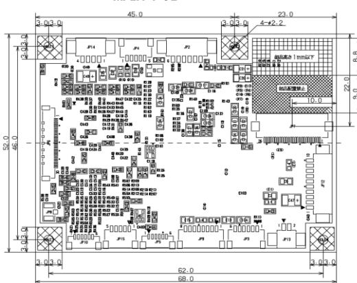
MAIN-PCB
