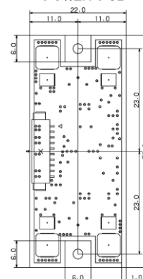
POWER-PCB
